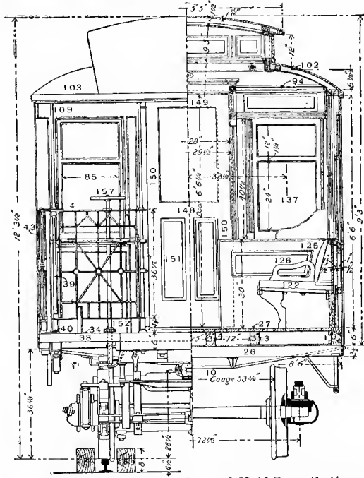
Fig. 466. Half End Elevation and Half Cross Section.
